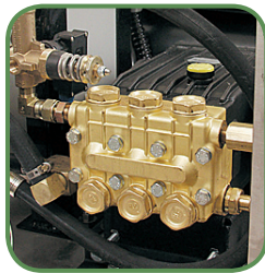
Pump accepts incoming water up to 175°F
